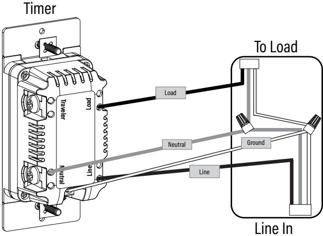
Typical Single-Pole Wiring
