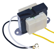
119T86A 24 VAC 20 VA Transformer, with #10 Ring Terminals
