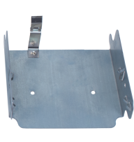
22T338GR Mounting Bracket for Intermatic Standardized Timer Mechanisms
