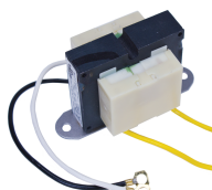
119T86A 24 VAC 20 VA Transformer, with #10 Ring Terminals
