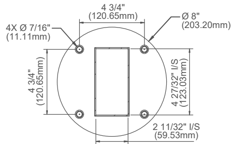
SINGLE GANG MODELS BASE MEASUREMENT
