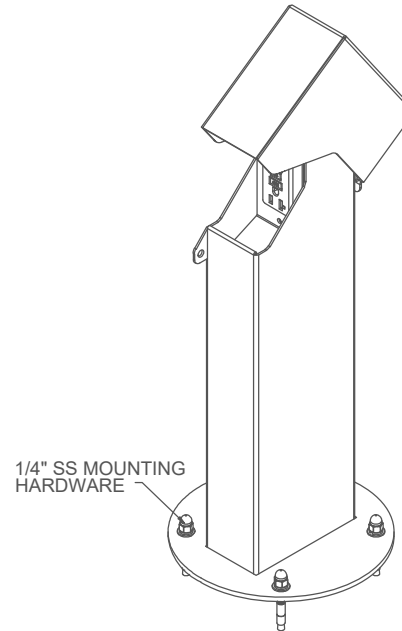
ISOMETRIC VIEW OPEN
